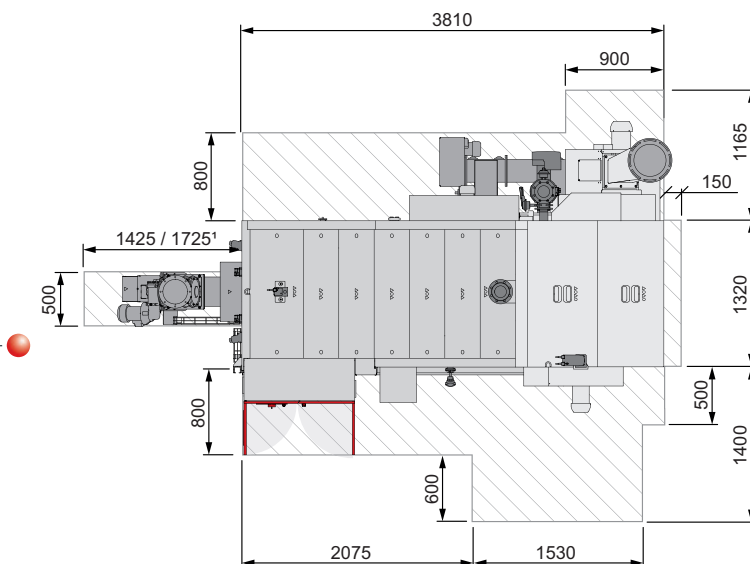
View of induced draught fan opposite the control cabinet
